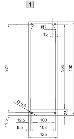
Mounting cut-out for external mounting
