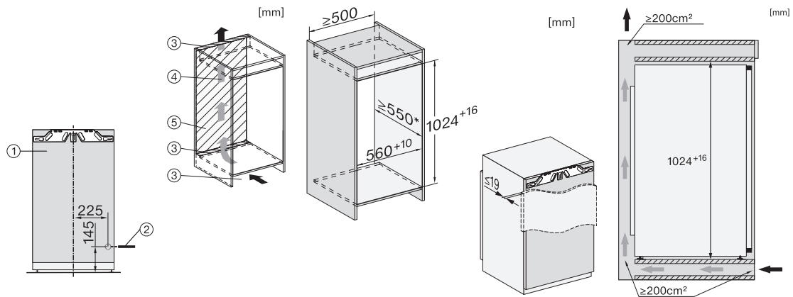
K7237D, K7238D, K7233E, K7234E, Installation (Fußnote*) (Skizze)
