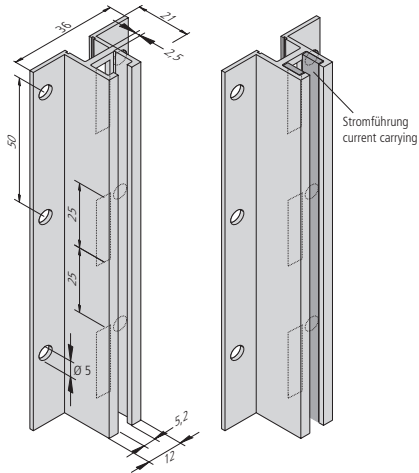
Schlitzschiene A Slotted rail A
