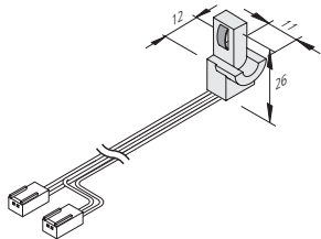
Endeinspeiser feeder element
