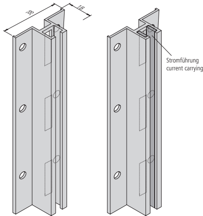
Schlitzschiene B Slotted rail B
