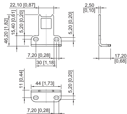
Angled actuator for safety switch
