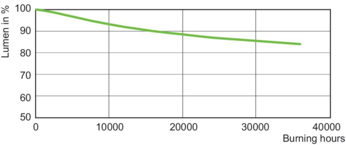
Lumen Maintenance Diagram - MST SON-T PIA Plus 400W E E40 1SL/12
