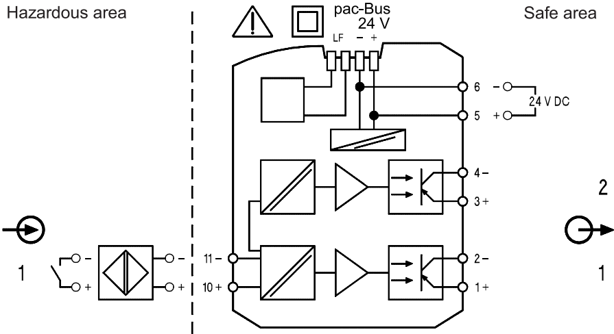
Connection diagram 9270/11-19-15
