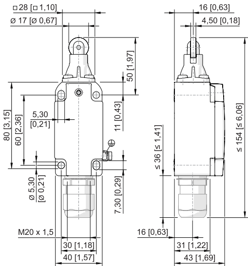
Roller plunger 8074/2-1-R-40
