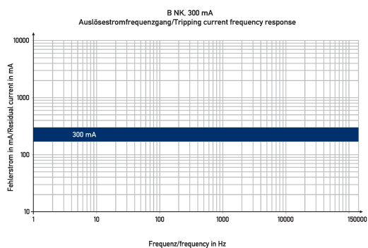
Diagramme FI-/LS-Kombinationen DRCBO 4 B16/o,30/3N-B NK
