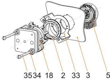
Front installation mounting with control switch series 8008
