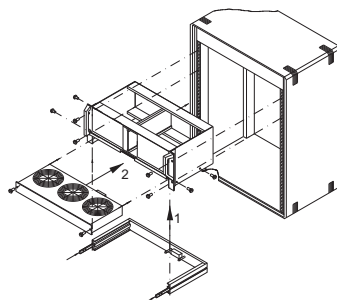
Schuifladeventilator Vario Montage in subracks 84 TE
