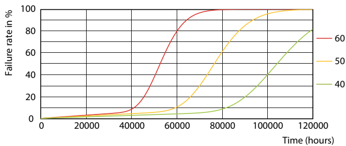
LEDtube_100K_4060_FailureRate-LED
