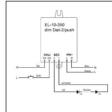
Connection for dim Dali2
