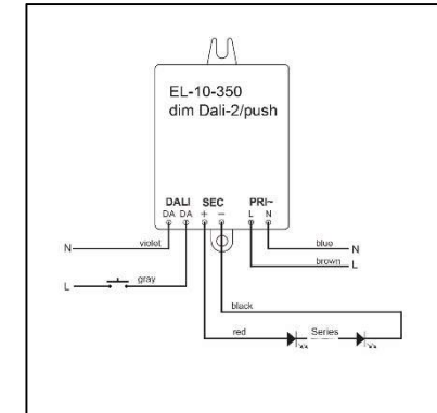
Connection for dim Push
