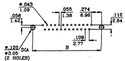
PCB HOLE PATTERNS
