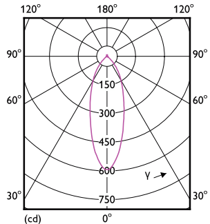
Light Distribution Diagram - MAS LED spot VLE DT 3.7-50W GU10 927 36D
