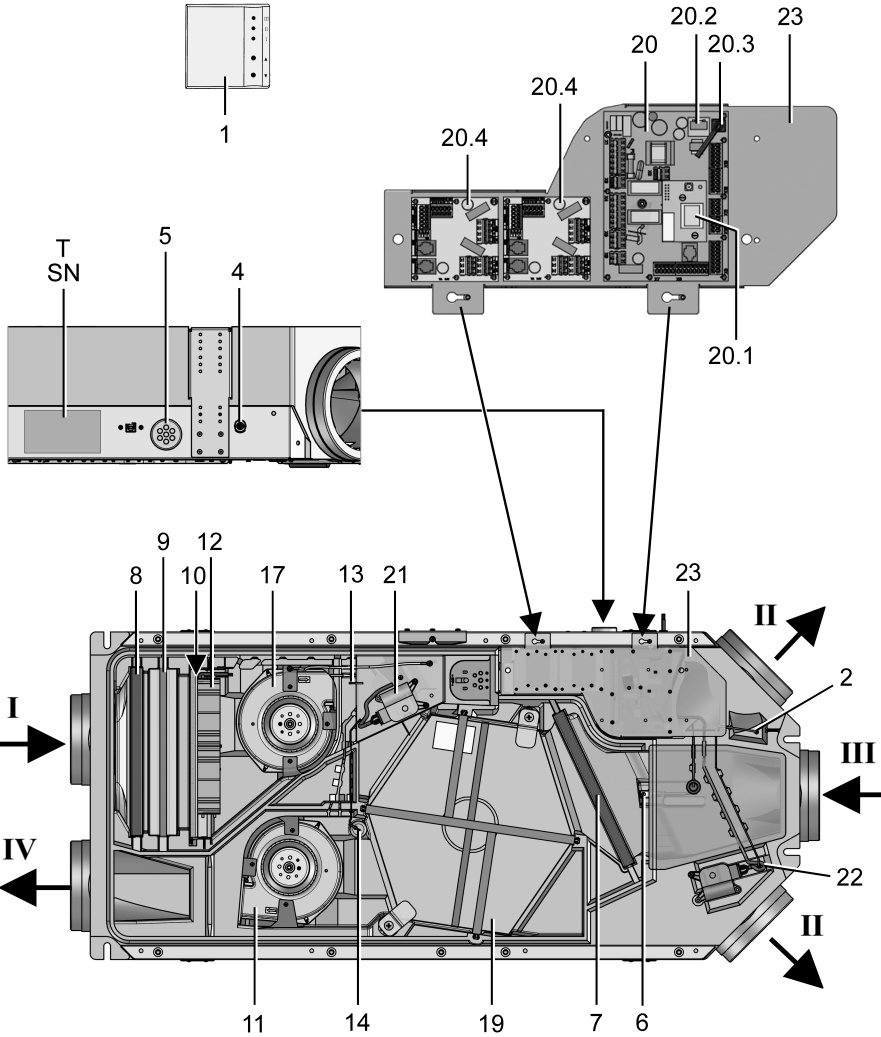
Figure : WS 160 Flat KBZET
