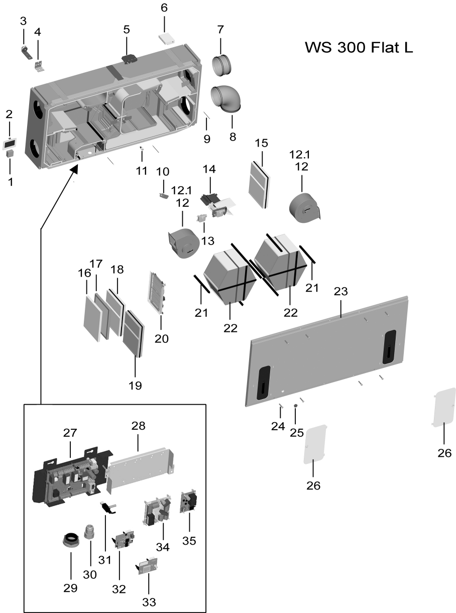
Figure = WS 300 Flat L Sans figure = version inversée WS 300 Flat R
