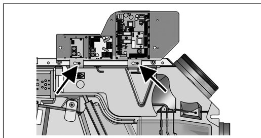
Arrow Fitting studs
