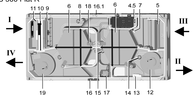
Figure: WS 300 Flat KBL/KBR (left-hand and right-hand versions)
