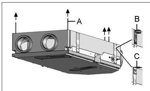
Mounting variants [A], [B] or [C]
