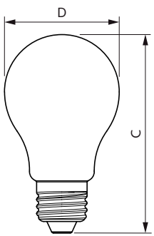
Bulb A60 230V 60W 806lm 2700-2200K E27
