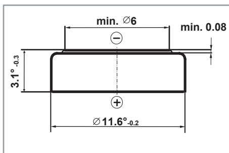
Diameter: 11.60 mm Height: 3.10 mm
