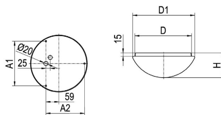
Maße [mm]
