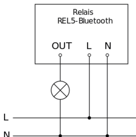
Circuit diagram 1
