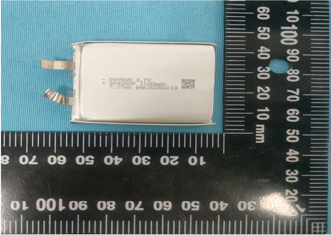
Figure 3 Overall view of cell (电芯外观图)
