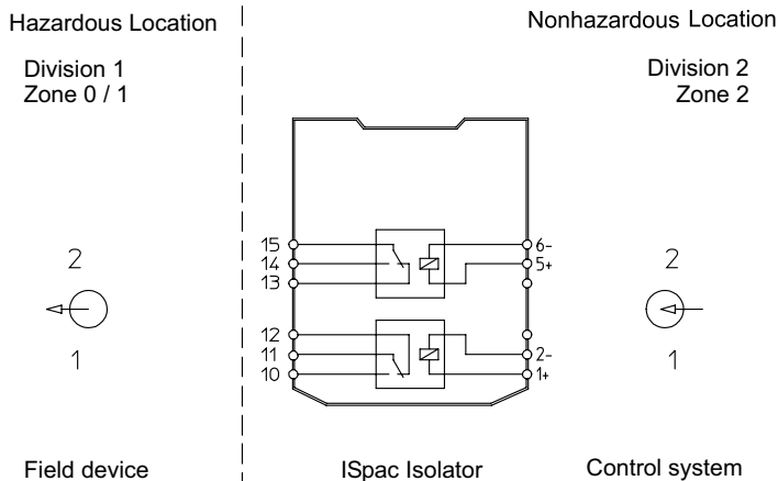
Connection Diagram 9172/21-11-00
