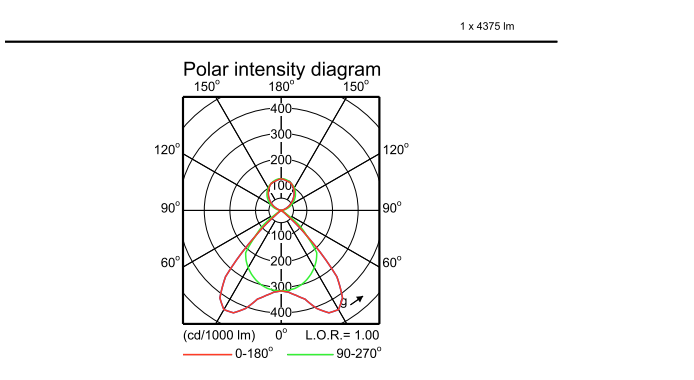
IFPC1_TPS642 1xTL5-49W HFP D8-VH.EPS
