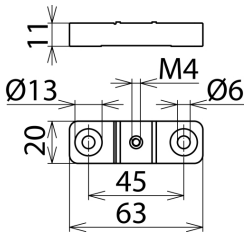
Maßbild ST AS SAK K
