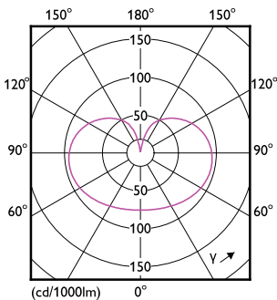
LEDbulb MAS SLR A60 10,5W E27 927 CL-LDD
