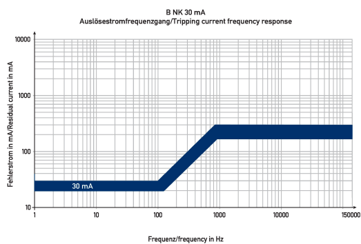
Diagramme FI-/LS-Kombinationen DRCBO 4 B16/o,03/1N-B NK
