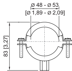
Mounting bracket for a thread
