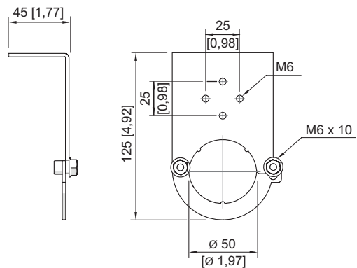
Mounting bracket for surfaces
