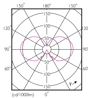
LEDBulb CLA 11-100W E27 A70 Clear 827 ND
