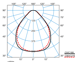
ArimoFit M84 PW19 42-840 ET + ArimoFit Sky M84-TS ZER TX426973
