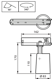
ST210T 39S/830 PSU MB BK
