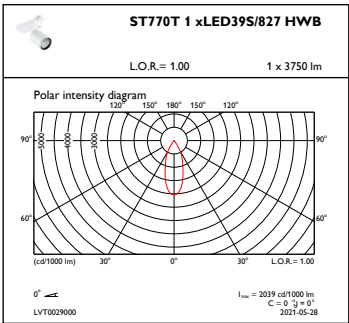
OFPC1_ST770T1xLED39S827HWB
