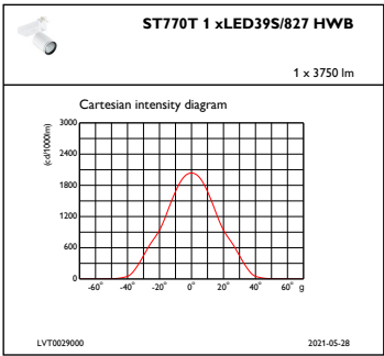
IFCC1_ST770T1xLED39S827HWB
