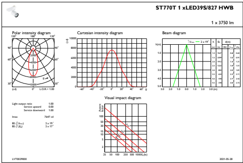
IFAS1_ST770T1xLED39S827HWB
