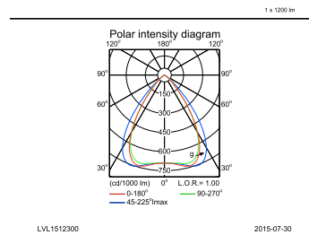
IFPC_DN572B PSE-E 1xLED12S/830 C-Polar Indoor (combined)
