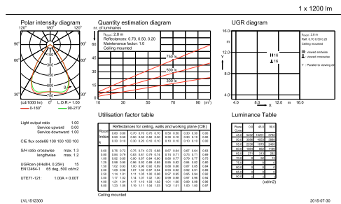
IFGU_DN572B PSE-E 1xLED12S/830 C-General uniform lighting
