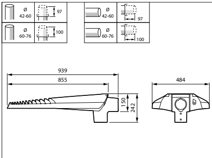
BGP705 LED300-4S/740 II DM11 GF SRT SRB
