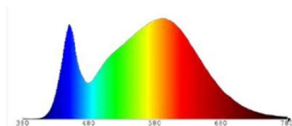
CCT - 4000K
