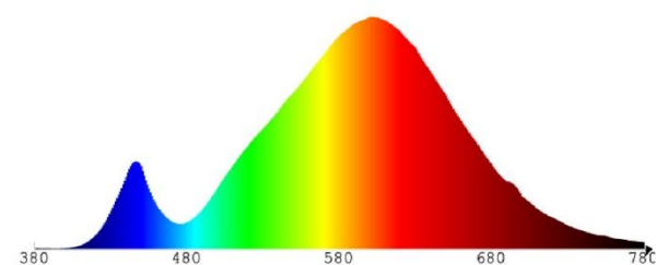
CCT - 3000K
