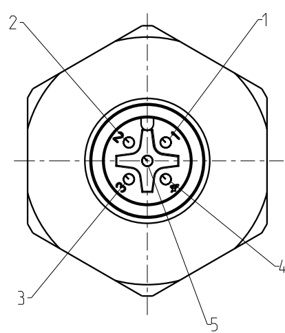
View of pin assignment Plug-in side
